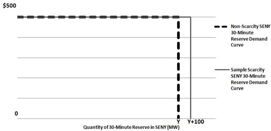
Example SENEY 30-Minute Reserve Demand Curve during a Real-Time Interval in which a 100 MW SENEY Scarcity Reserve Requirement is Established
