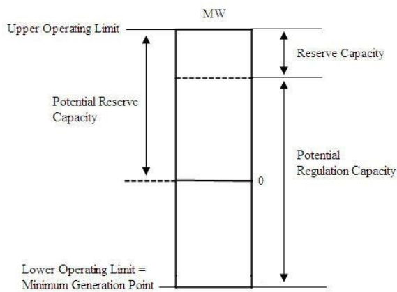
Figure 5: Demand Side Resources Operating Characteristics
